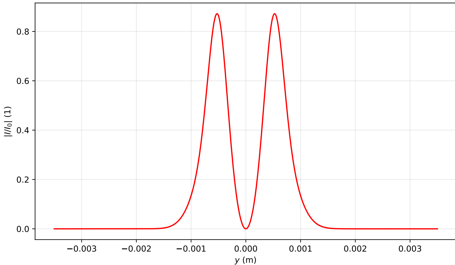
Intensity profile I(x=0, y, z=0.557)/I_0 , P_{in}=3.0P_{cr} , artificial time
